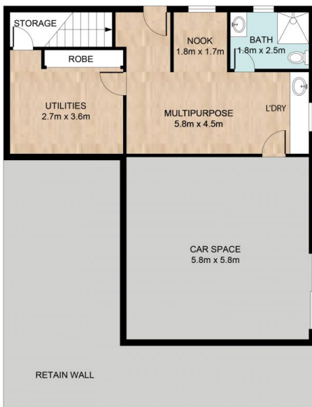
GROUND LEVEL
